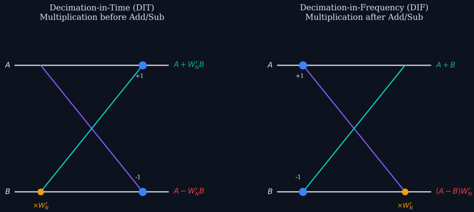
Figure 1: Large FIR filters can be implemented efficiently using block convolution methods which rely on the Fast Fourier Transform (FFT). The butterfly structure of the FFT is shown.
