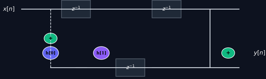
Symmetric Linear-Phase FIR folding structure ( M = 4 )
