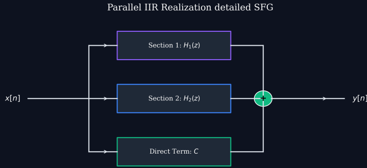
Figure 1: Parallel IIR Signal Flow Graph.
