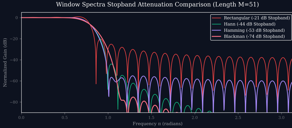
Figure 2: Sidelobe Suppression
