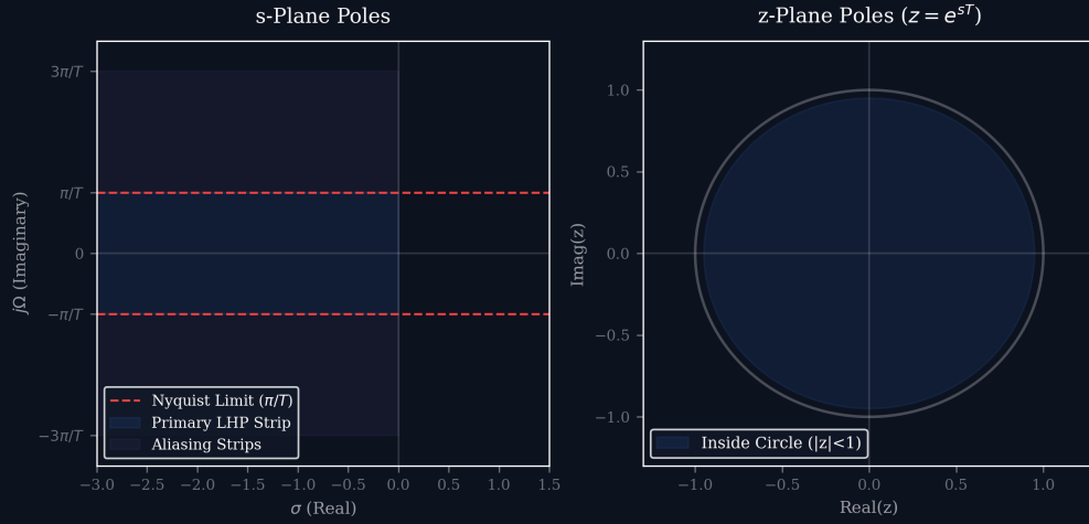
Figure 1: Impulse Invariance Mapping
