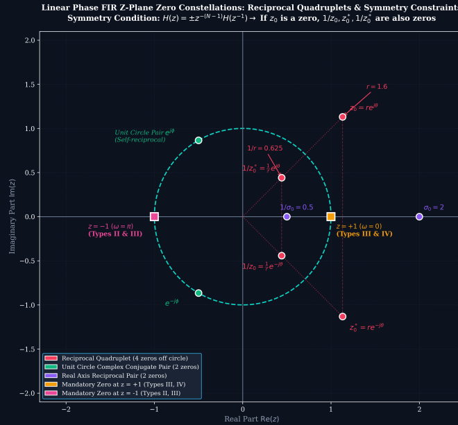
Figure 1: Zero constellations for linear-phase FIR systems: complex quadruplets off the unit circle, pairs on the unit circle ( |z| = 1 ), and mandatory boundary zeros at z = \pm 1 .
