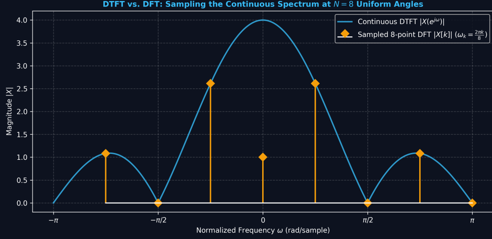
Figure 1: Sampling the Continuous DTFT Spectrum at N = 8 Uniform Frequency Angles \omega_k = \frac{2\pi k}{8} .
