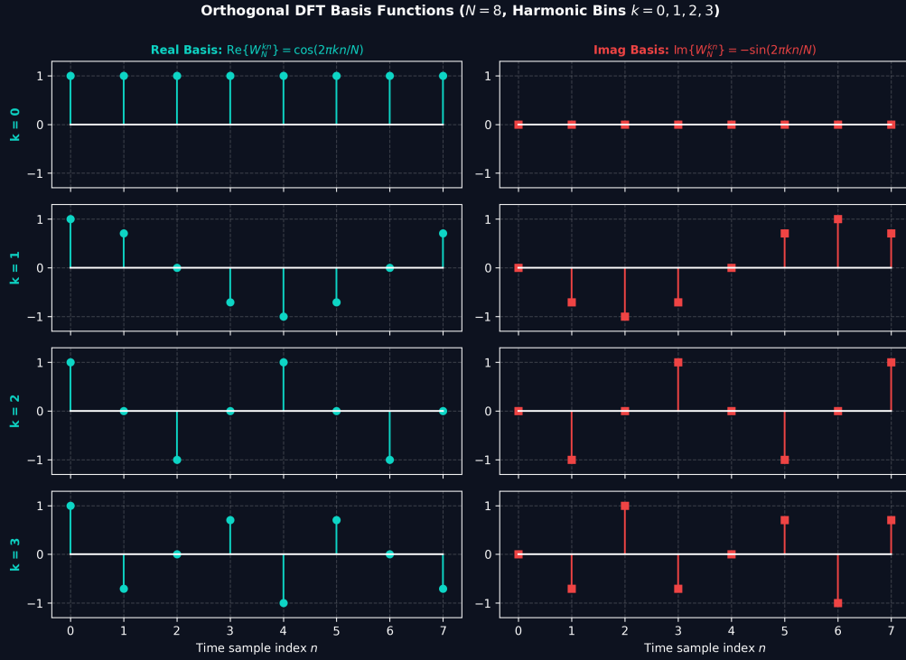
Figure 2: Orthogonal Real (Cosine) and Imaginary (Sine) DFT Harmonic Basis Functions for N = 8 .
