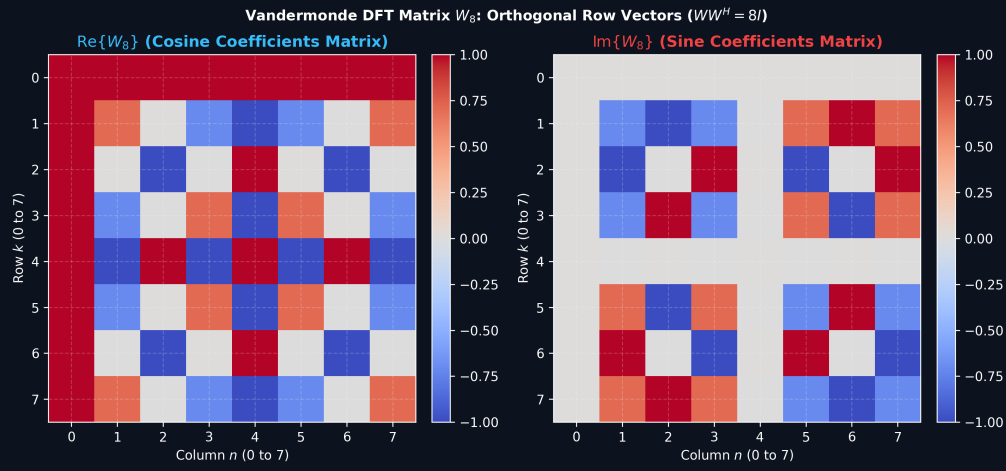
Figure 3: Vandermonde DFT Matrix W_8 : Visualizing Real and Imaginary Orthogonal Matrix Coefficients.
