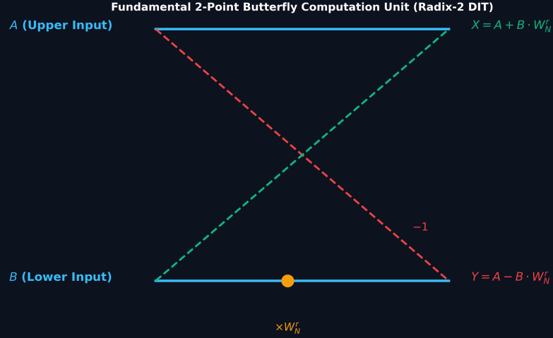
Figure 3: Fundamental 2-Point Butterfly Computation Unit (Radix-2 DIT).
