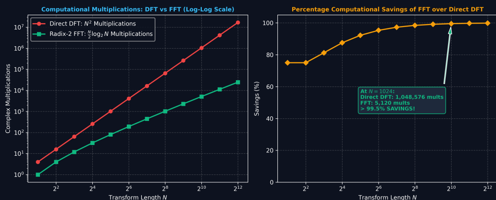
Figure 1: Computational Scaling: Direct DFT O(N^2) vs. Radix-2 FFT O(N \log_2 N) (> 99.5% Savings for N = 1024 ).
