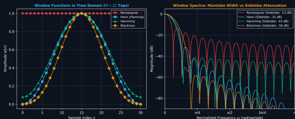
Figure 1: Window Functions in Time and Frequency Domains: Mainlobe Width vs. Sidelobe Attenuation Trade-offs.
