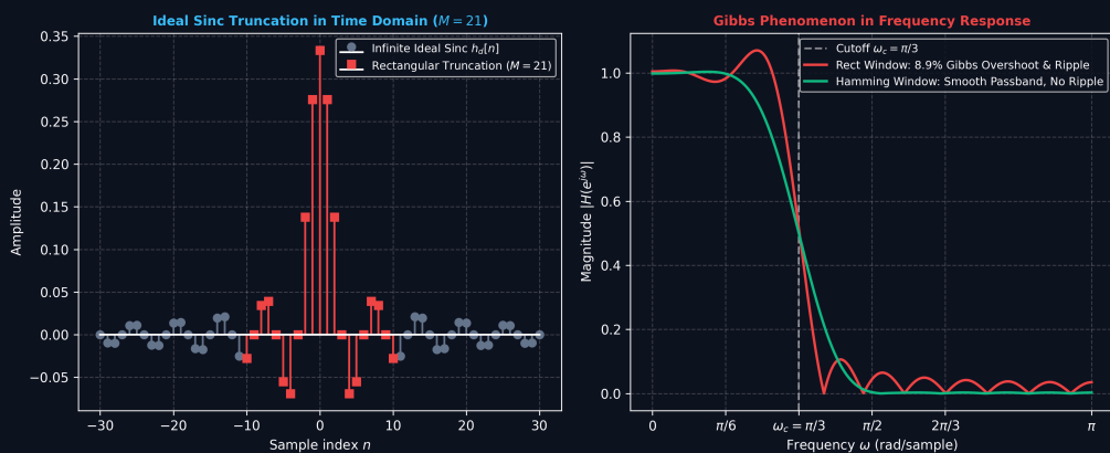
Figure 2: Gibbs Phenomenon: Abrupt Truncation Overshoot (8.9%) vs. Smooth Hamming Window Suppression.
