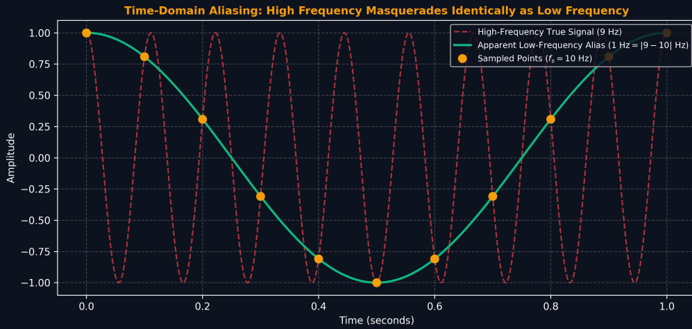
Figure 2: Time-Domain Aliasing: High-Frequency Sine Wave Masquerading Identically as a Low-Frequency Alias.
