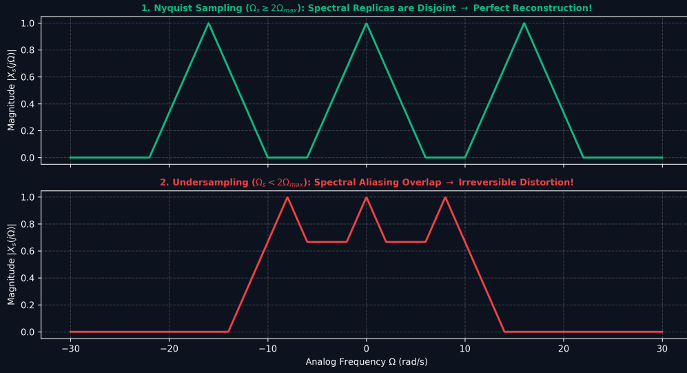
Figure 1: Sampling in the Frequency Domain: Spectral Replication and Aliasing Overlap when \Omega_s < 2\Omega_{max} .
