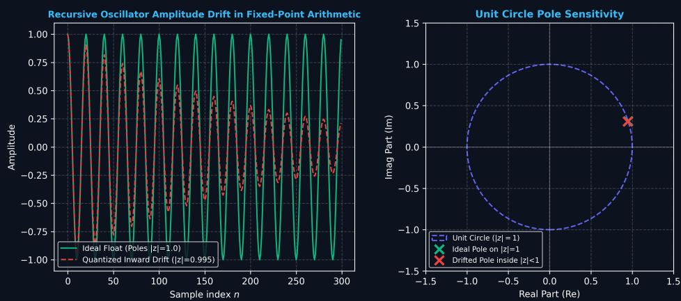
Figure 1: Fixed-Point Coefficient Sensitivity: Unit-Circle Pole Quantization Drift and Amplitude Instability.
