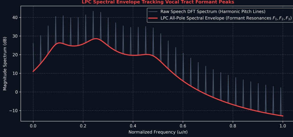
Figure 2: Linear Predictive Coding (LPC) Spectral Envelope Tracking Vocal Tract Formant Resonances ( F_1, F_2, F_3 ).
