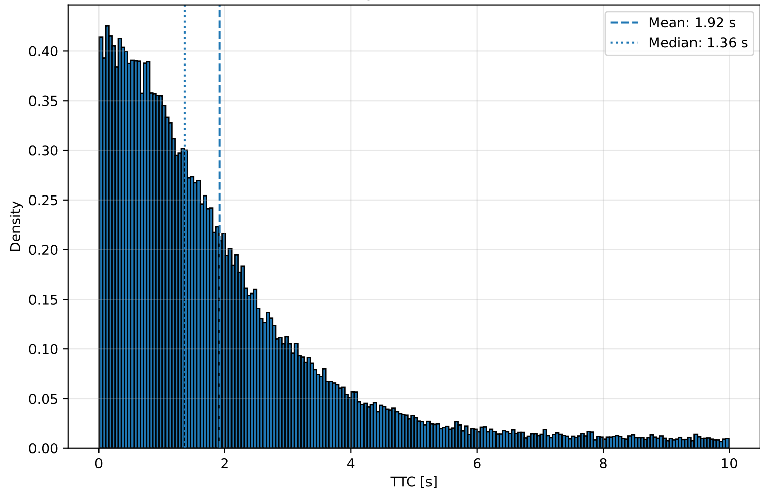
TTC to Target-Lane Front Vehicle
