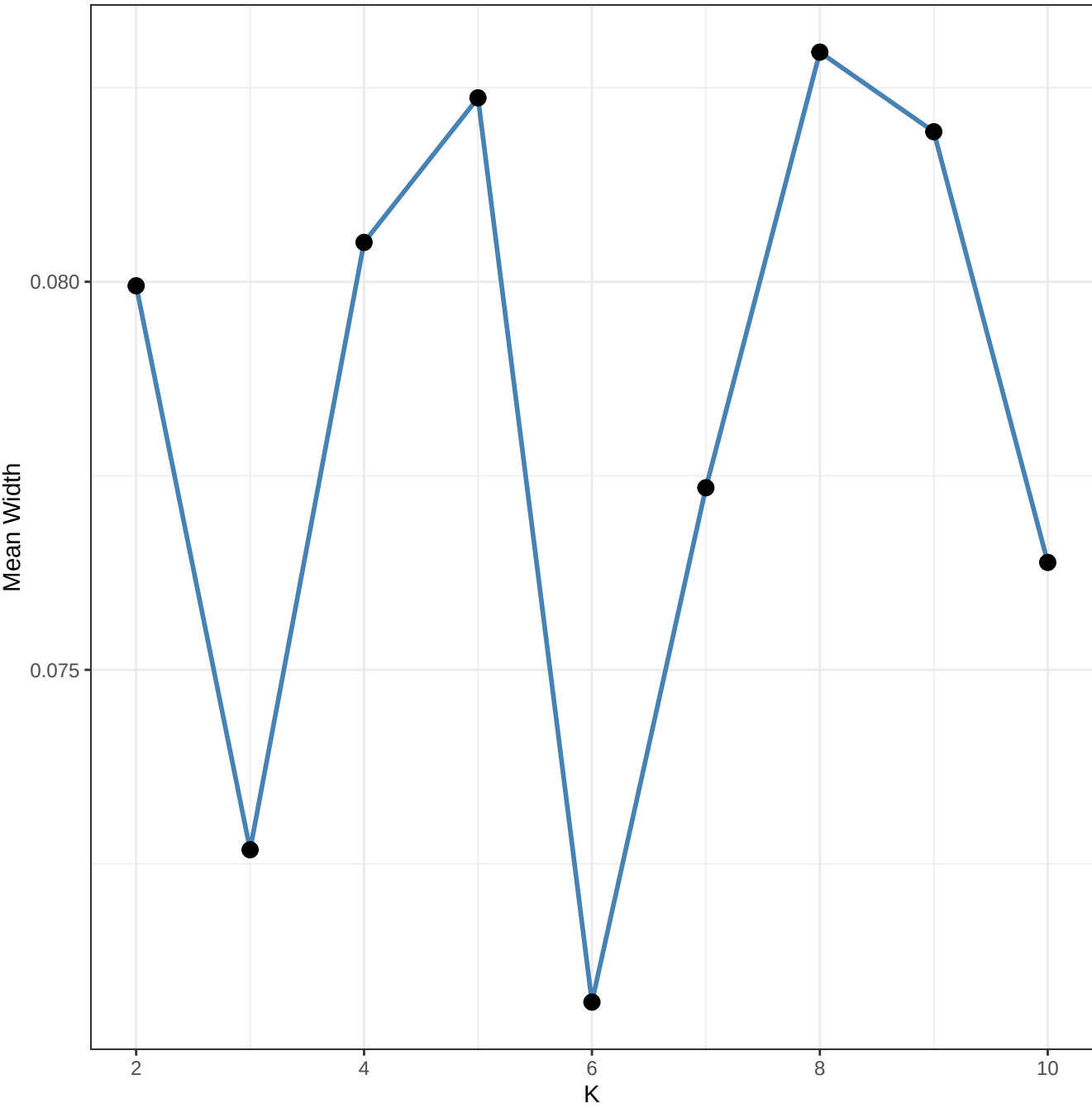
Silhouette Score Higher = Better Separation
