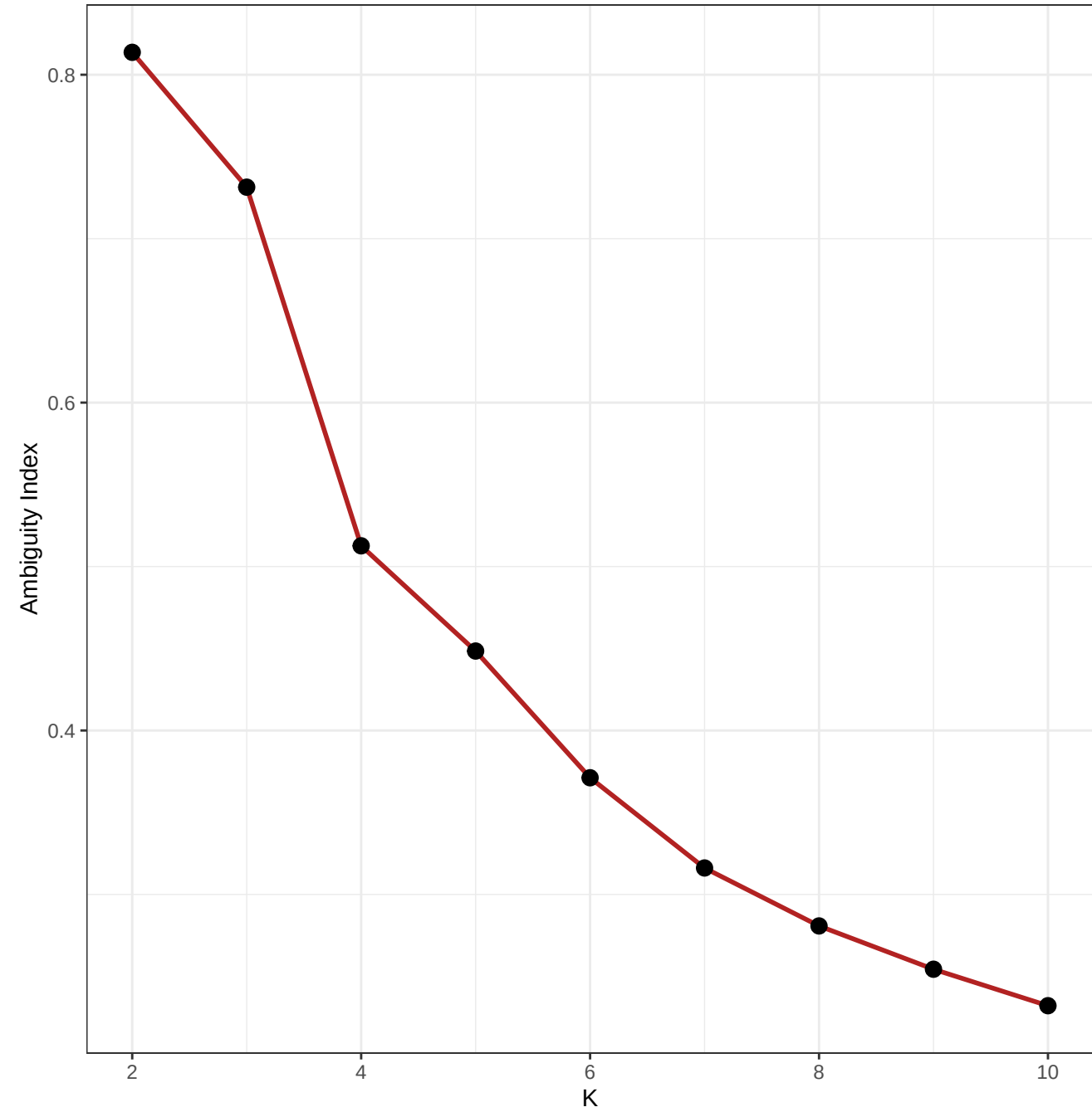
PAC Score Lower = Most Stable Clusters
