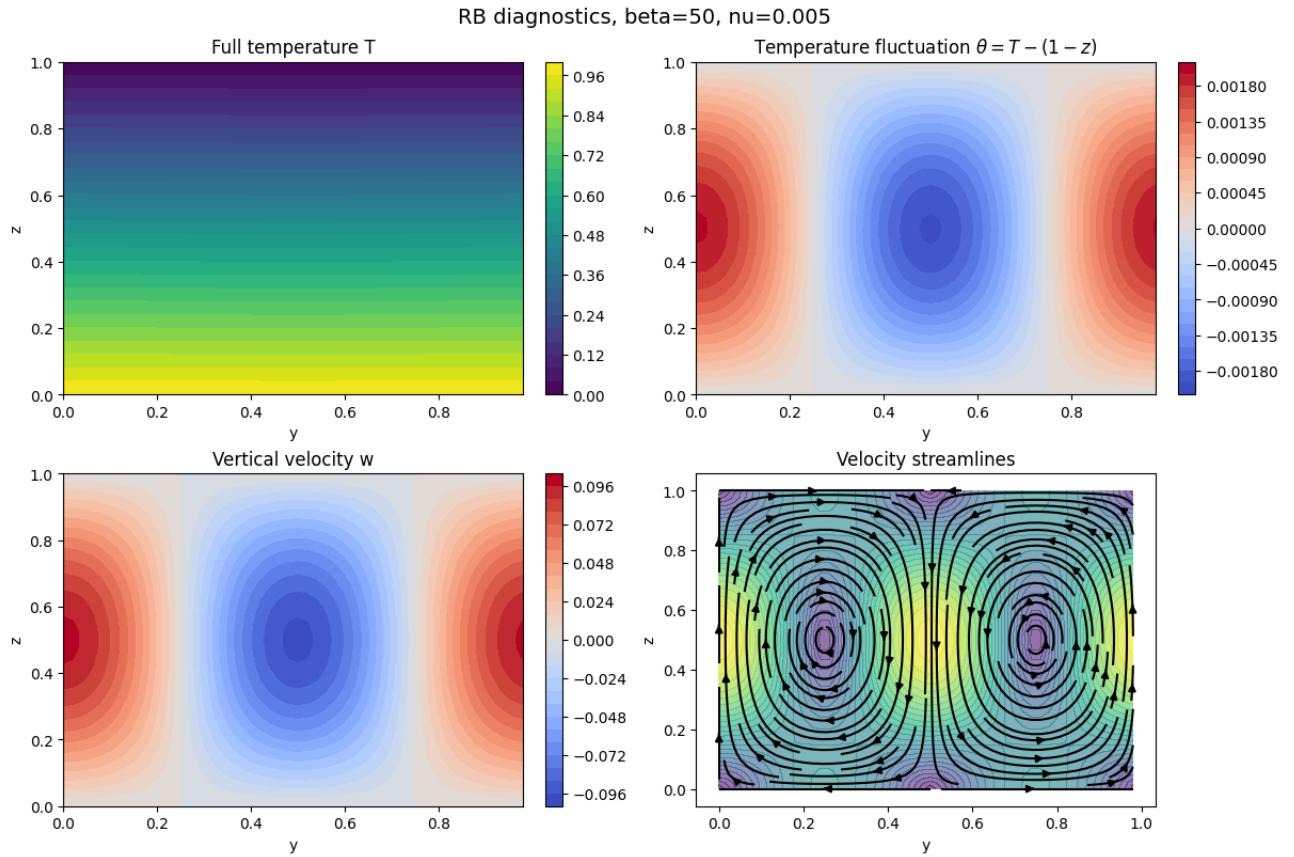
Figure 3.5: Results of the numerical solution for \beta = 50 , \nu = 0.005 . Results for a parameterisation causing Rayleigh-Bénard convection cells induced by thermal forcing (for thermal forcing see plot at the upper left).
