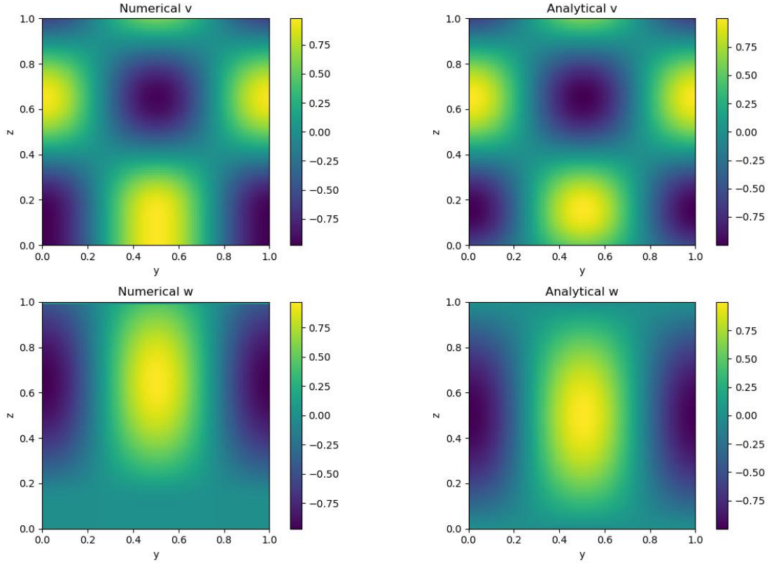
Figure 3.1: Comparison of analytical and numerical solutions in advection test.
