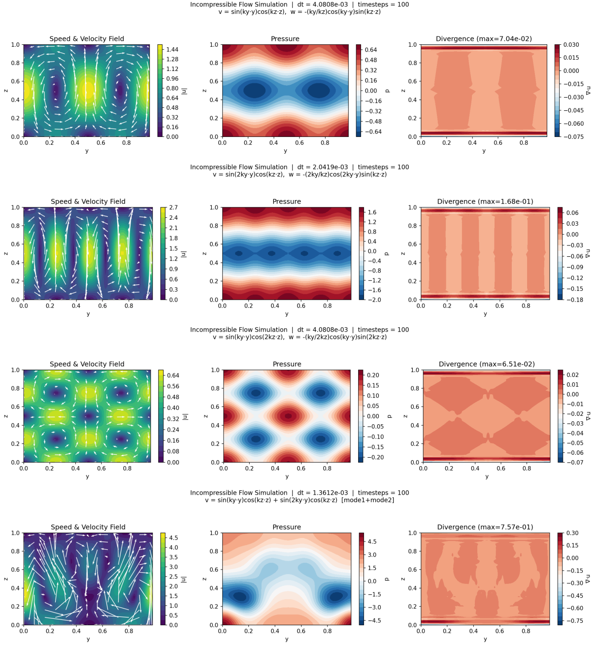
Figure 3.2: Resulting simulation results. Flow behavior for different parameterisations. Numerical calculations have been performed by using FFT and spectral decomposition.
