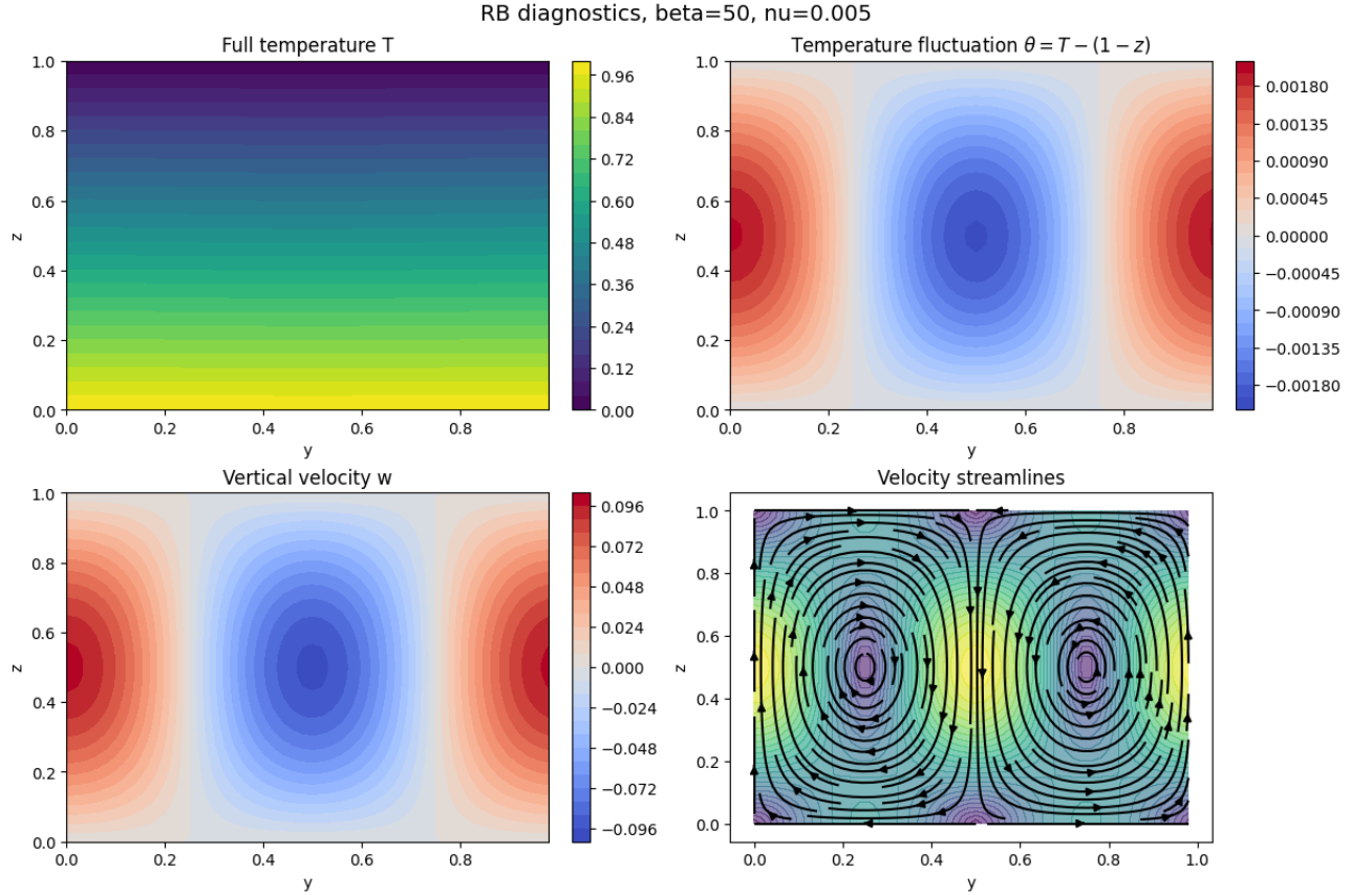
Figure 3.5: Results of the numerical solution for \beta = 50 , \nu = 0.005 . Results for a parameterisation causing Rayleigh-Bénard convection cells induced by thermal forcing (for thermal forcing see plot at the upper left).
