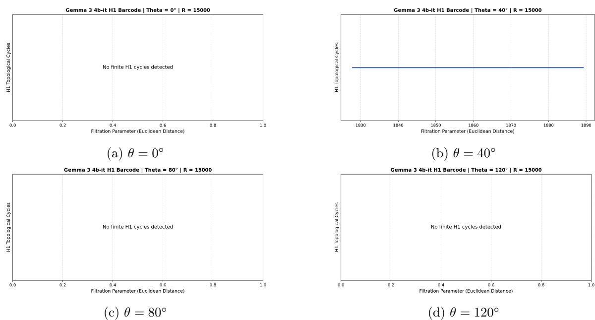
Figure 14.1: Representative H_1 Persistent Homology Barcodes for K = 0 . The flat lines or empty diagrams mathematically confirm the contractibility of the generation path.
