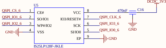
Flash memory
