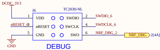
Probe connector
