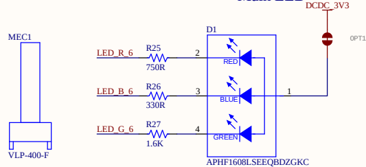
Main LED
