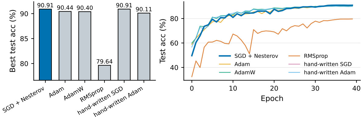
Figure 2: Optimizer ablation on the ConvNet: best test accuracy (left) and test-accuracy curves (right).
