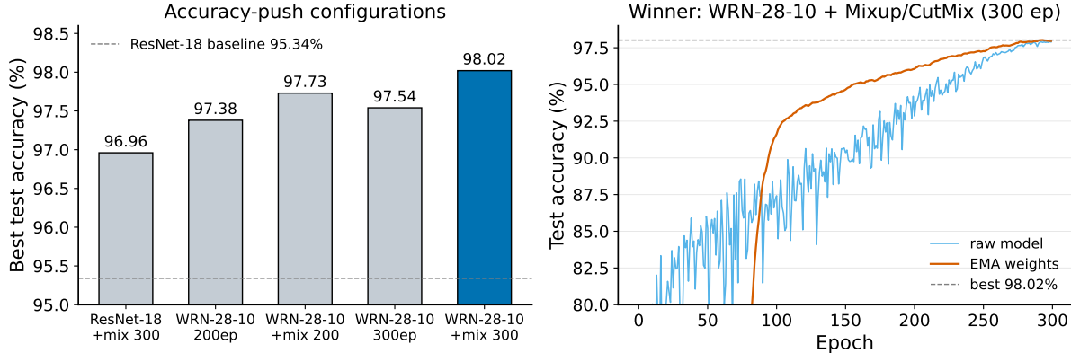
Figure 3: Left: best test accuracy of the five high-accuracy configurations vs. the ResNet-18 baseline (95.34%, dashed). Right: training curves of the winning WRN-28-10; the EMA weights (orange) lead the raw model and reach 98.02%.
