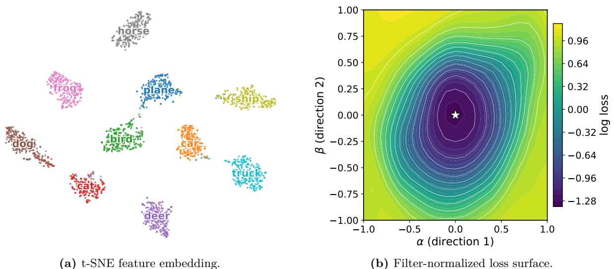
Figure 4: Diagnostics for the best CIFAR-10 model. The diagnostics show feature separability and local loss geometry without repeating the ablation comparisons.
