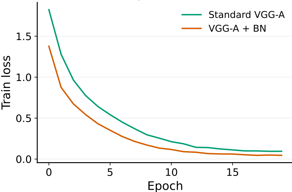
Training loss (lr=0.001)
