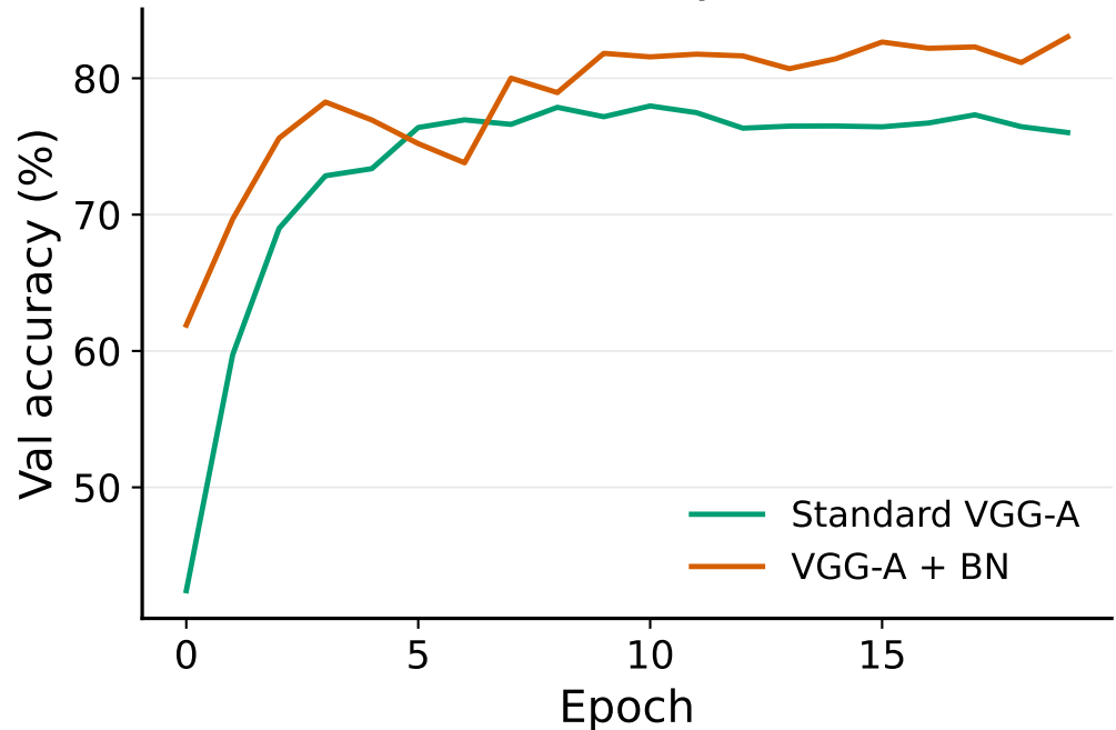
Validation accuracy (lr=0.001)
