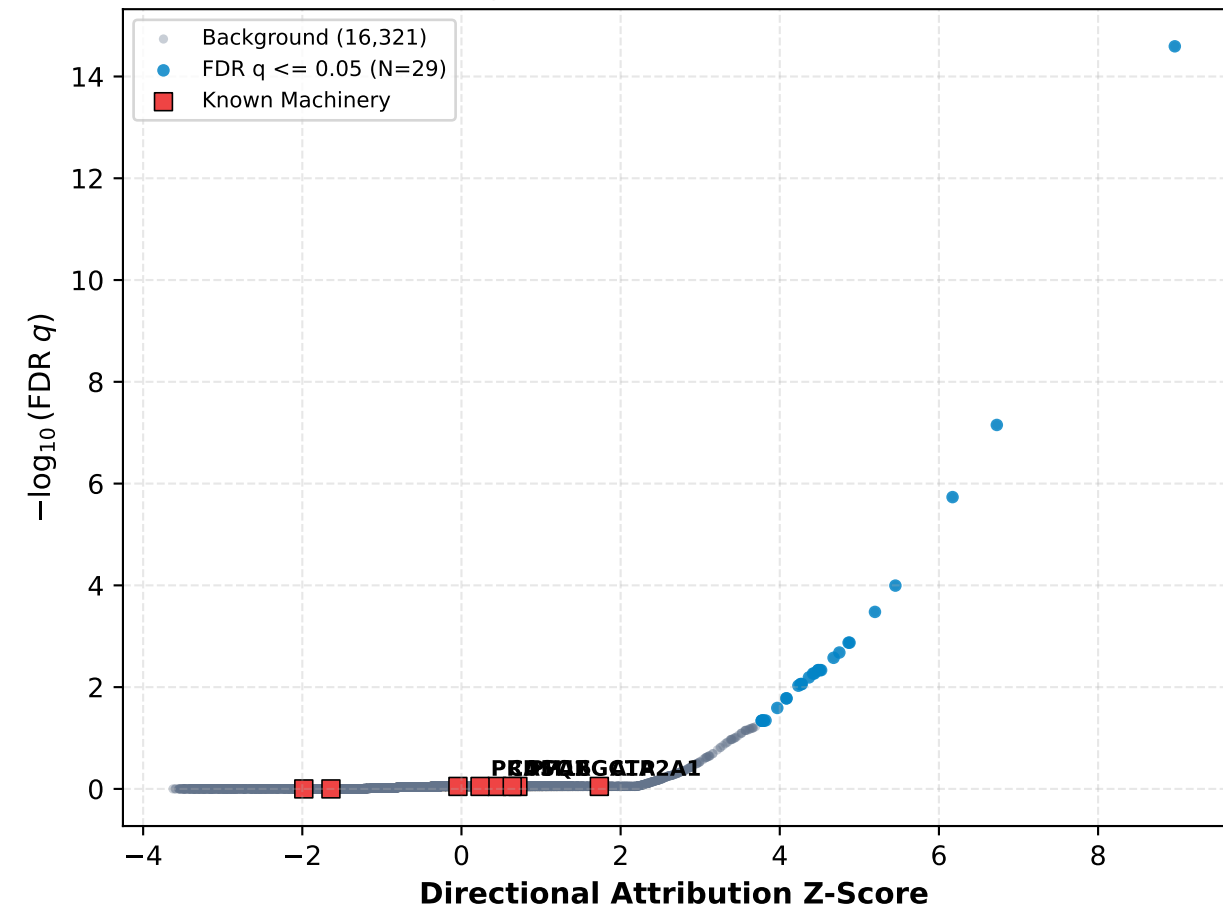
A) Whole-Genome Screening: Loss of UCP1 & Brown Adipose Thermogen
