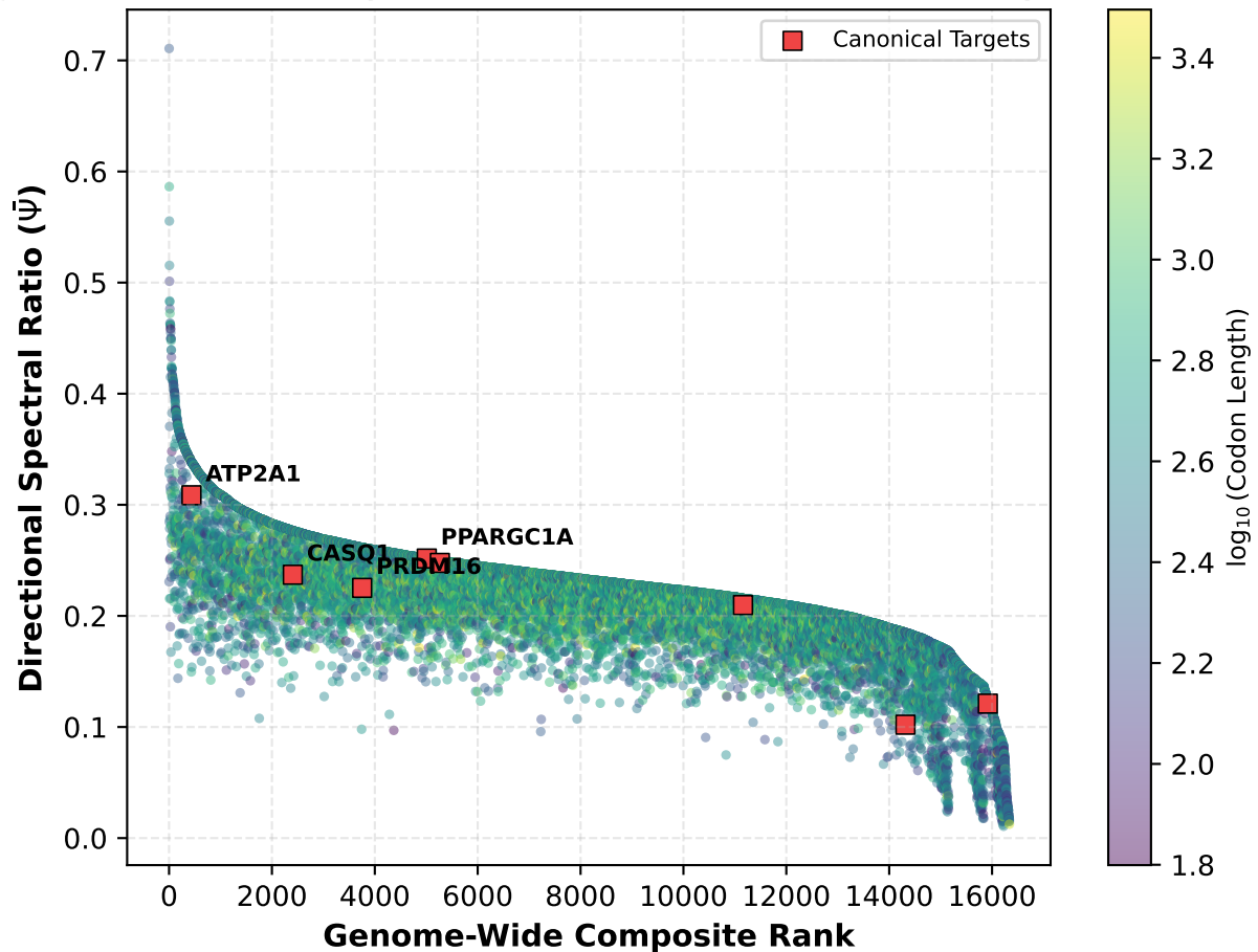
genesis(B) Discovery Landscape & Canonical Machinery
