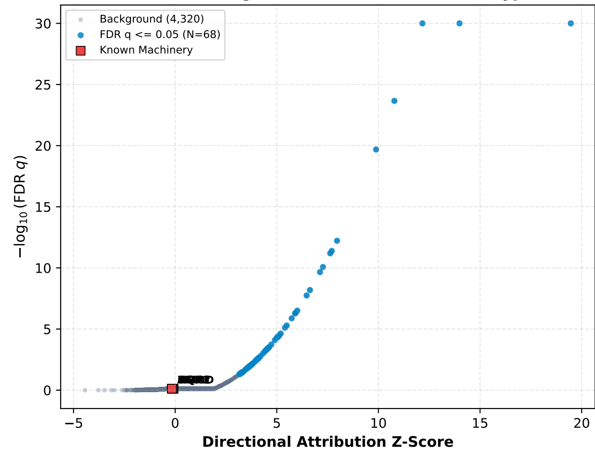
A) Whole-Genome Screening: Subterranean / Fossorial Hypoxia Adaptation
