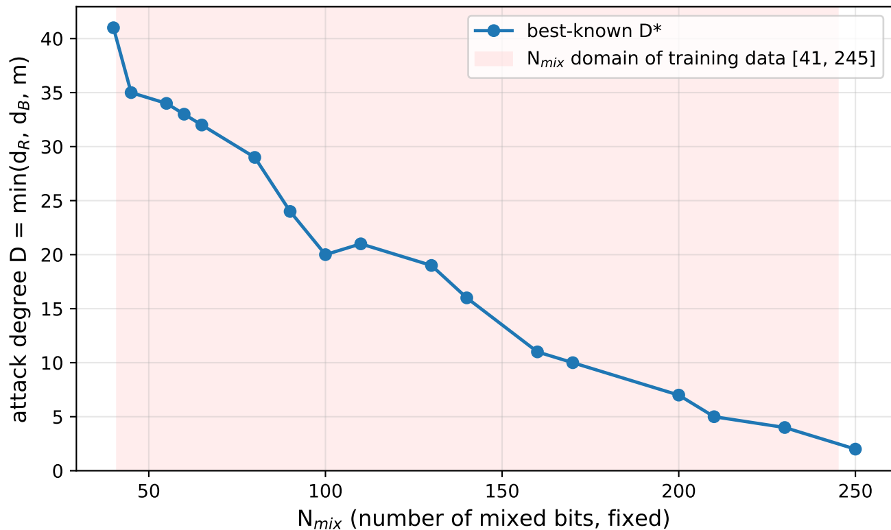
N_{mix} vs. attack degree (SHA3-512)
