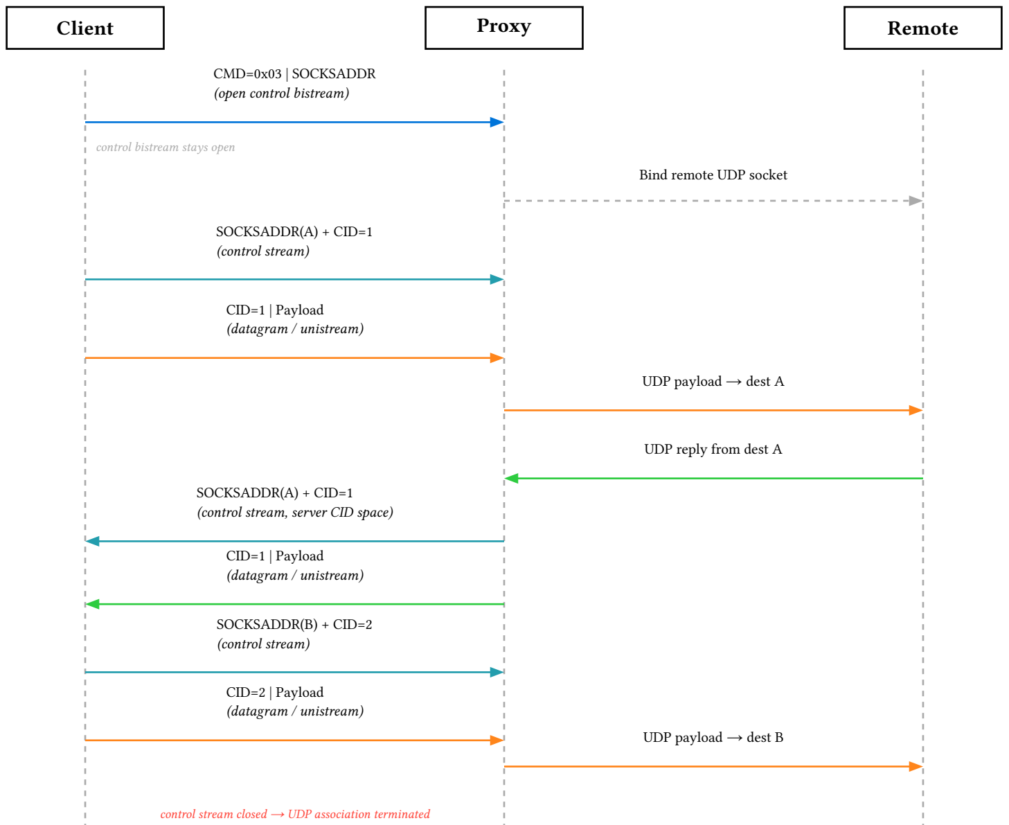
Figure 1: UDP Association data transfer process
