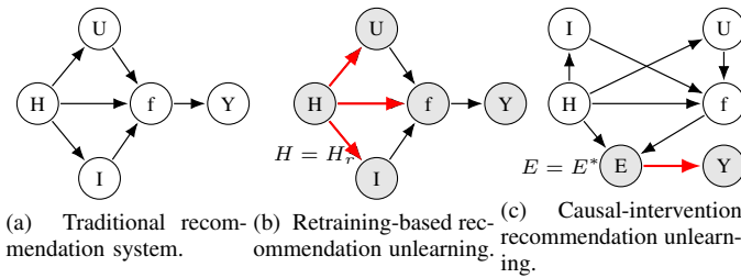
Fig. 2. Causal graphs for recommendation unlearning. Nodes denote H (historical interactions), U (users), I (items), f (model), E (explanation), and Y (output). (a) Standard recommendation SCM. (b) Retraining-based unlearning through do(H := H_r) . (c) CEU with a localized intervention on the E \rightarrow Y path, approximating the removal of forgotten-data effects without modifying f .
