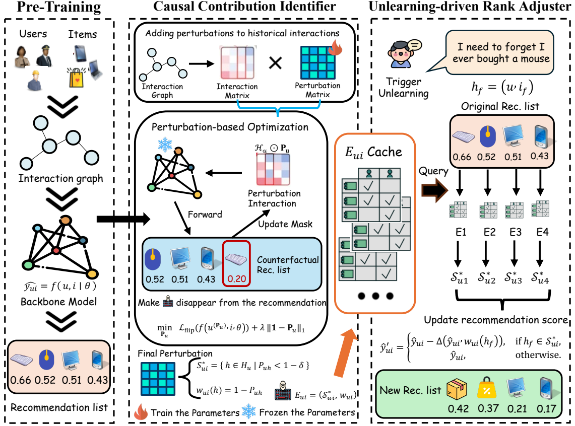
Fig. 3. The framework of CEU. The Pre-Training pipeline generates the initial ranking results. The Causal Contribution Identifier identifies the minimal causal support set and quantifies their contribution to the recommendation. The Unlearning-driven Rank Adjuster performs localized score adjustment to remove the influence of the forgotten interaction.
