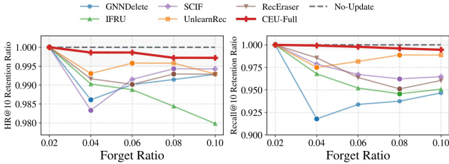
Fig. 6. Retained-set stability under increasing forget ratios. The left panel shows the HR@10 retention ratio, and the right panel shows the Recall@10 retention ratio, both normalized by the value at the 2% forget ratio. Higher values indicate better retained-set stability under stronger forgetting.
