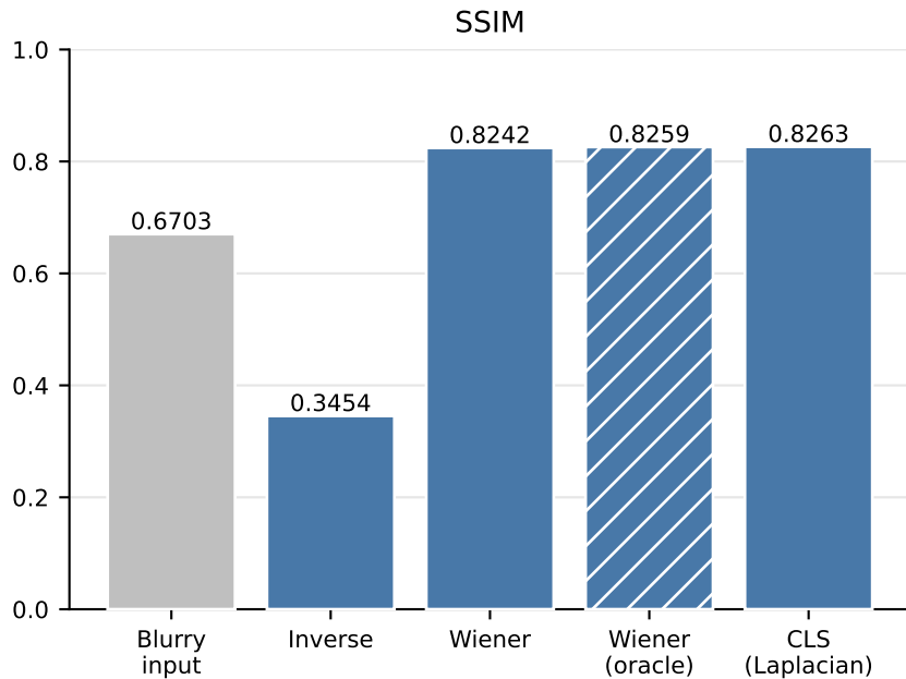
Fourier-domain restoration, CBSD68 ( \sigma = 2 , 68 images); hatched = oracle
