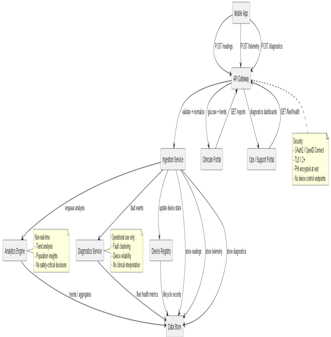
CGMS Cloud API Interface (Updated)
