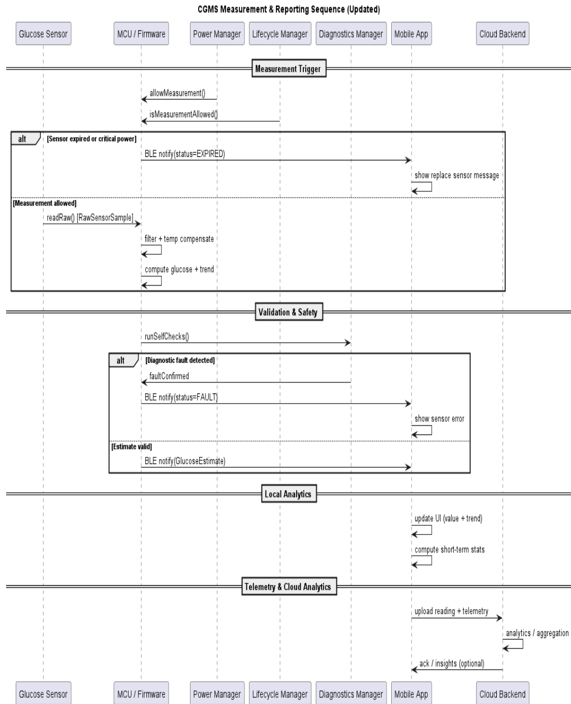
Sequence Diagram
