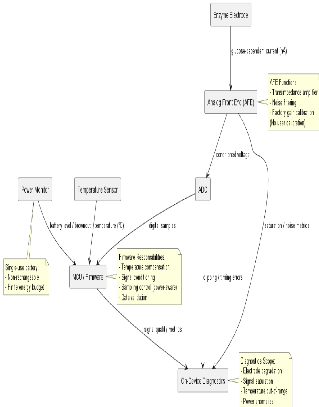
CGMS Sensor Interface (Updated)
