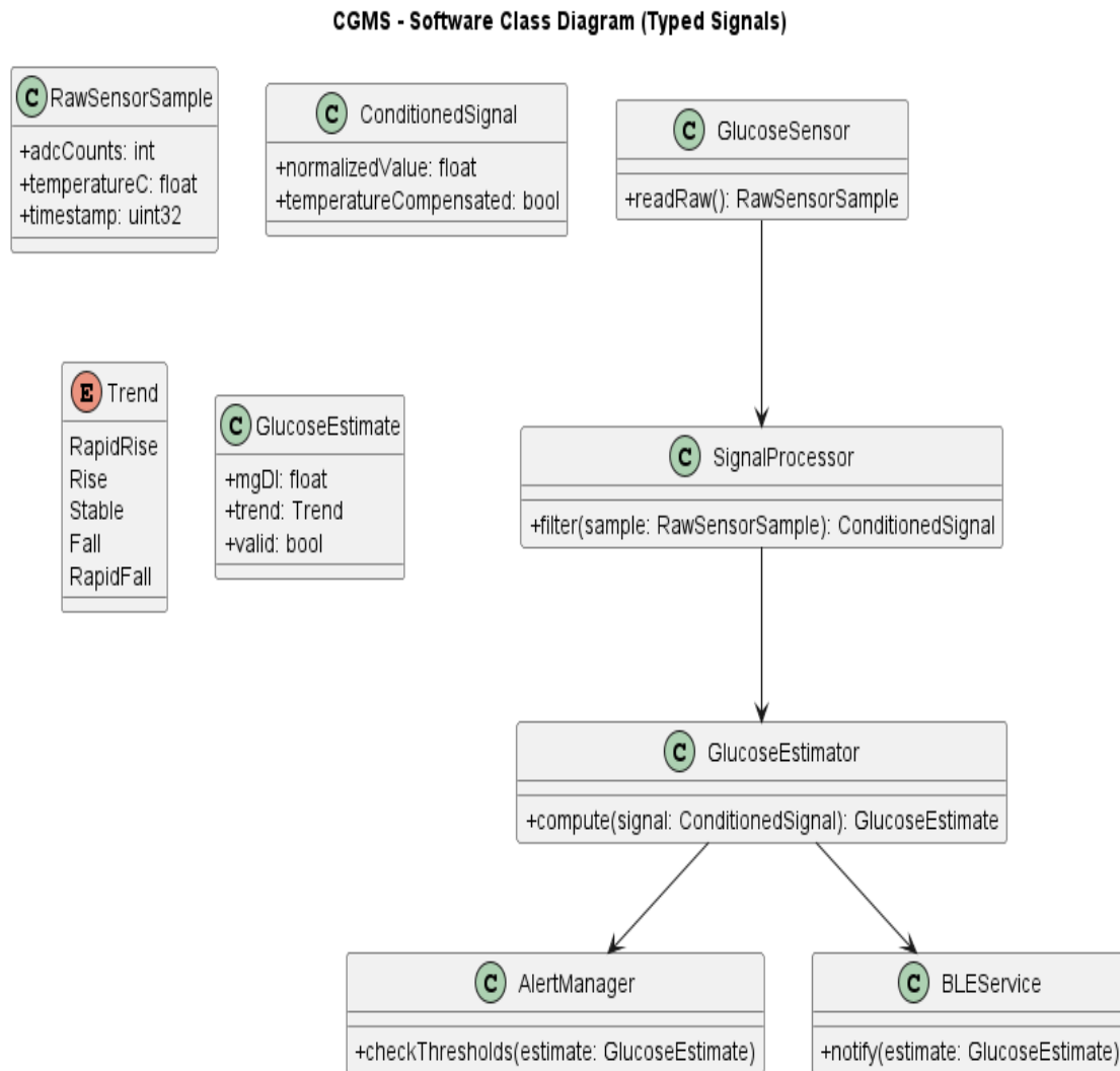
Class Diagram
