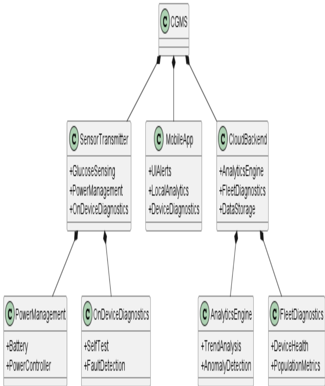
CGMS - Block Definition Diagram (BDD)
