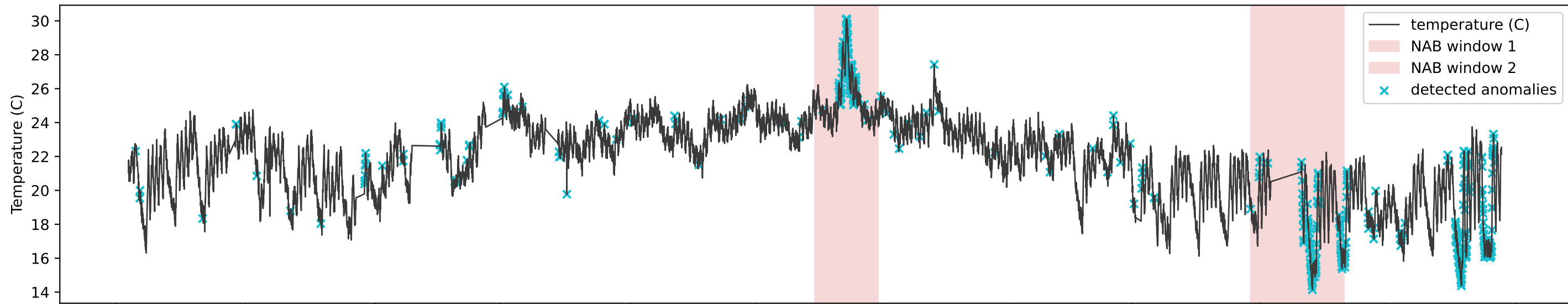
Best Tuned Hybrid OR - MP@p99 OR Z@p99 OR IF@p95 (A) NAB windows vs detector alarms
