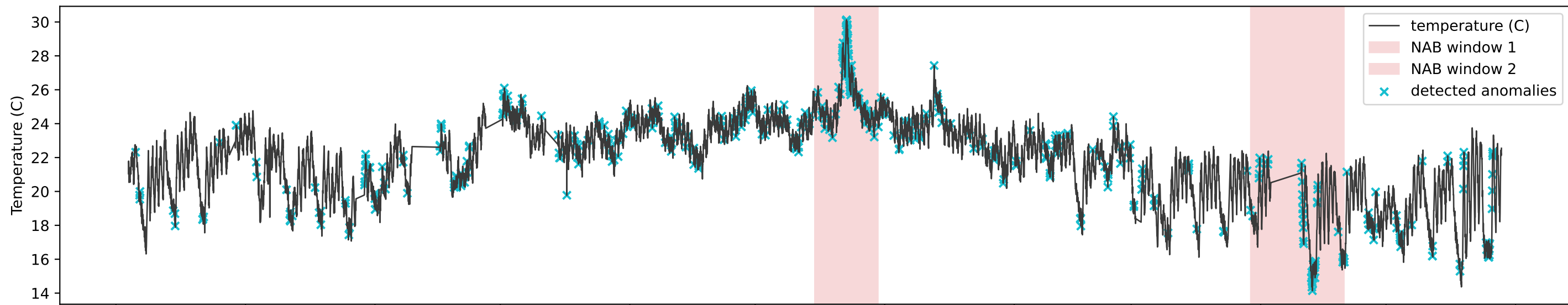
Hybrid OR - Matrix Profile p95 OR Rolling Z-score p99 OR Isolation Forest p99 (A) NAB windows vs detector alarms
