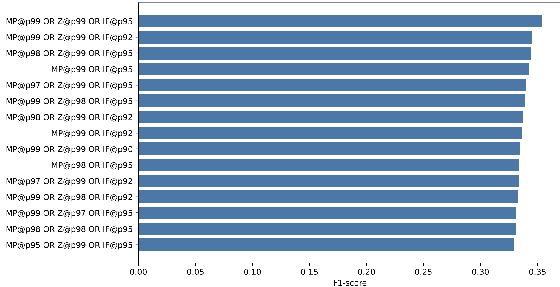
Top-15 Hybrid OR configurations by F1
