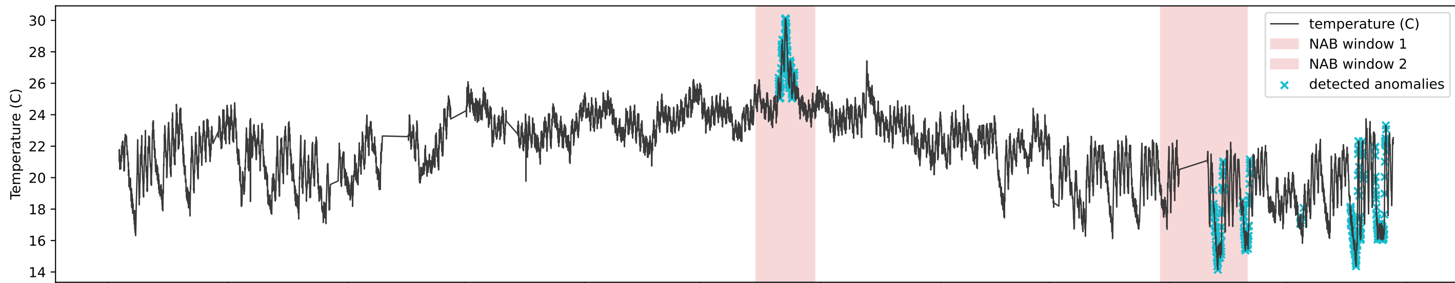
Isolation Forest - GT vs Detected (window=48h, p95) (A) NAB windows vs detector alarms
