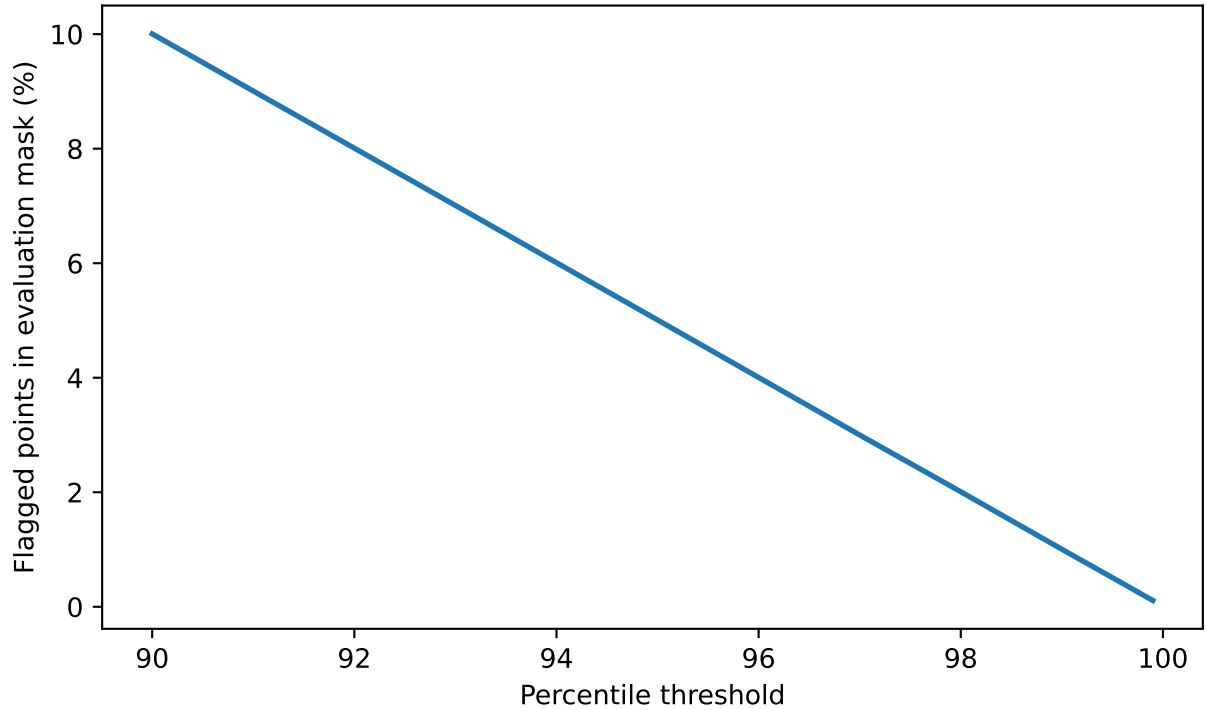
Isolation Forest - Percentile Sweep (window=48h): Alarm rate vs percentile threshold
