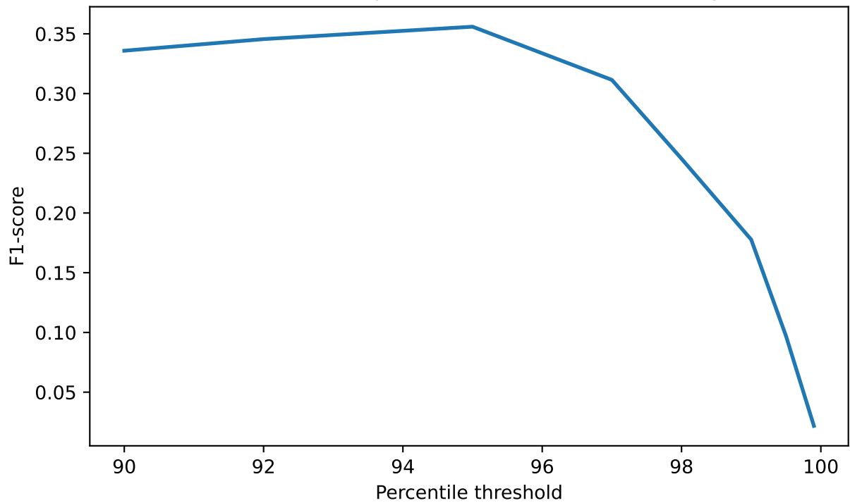
Isolation Forest - Percentile Sweep (window=48h): F1-score vs percentile threshold
