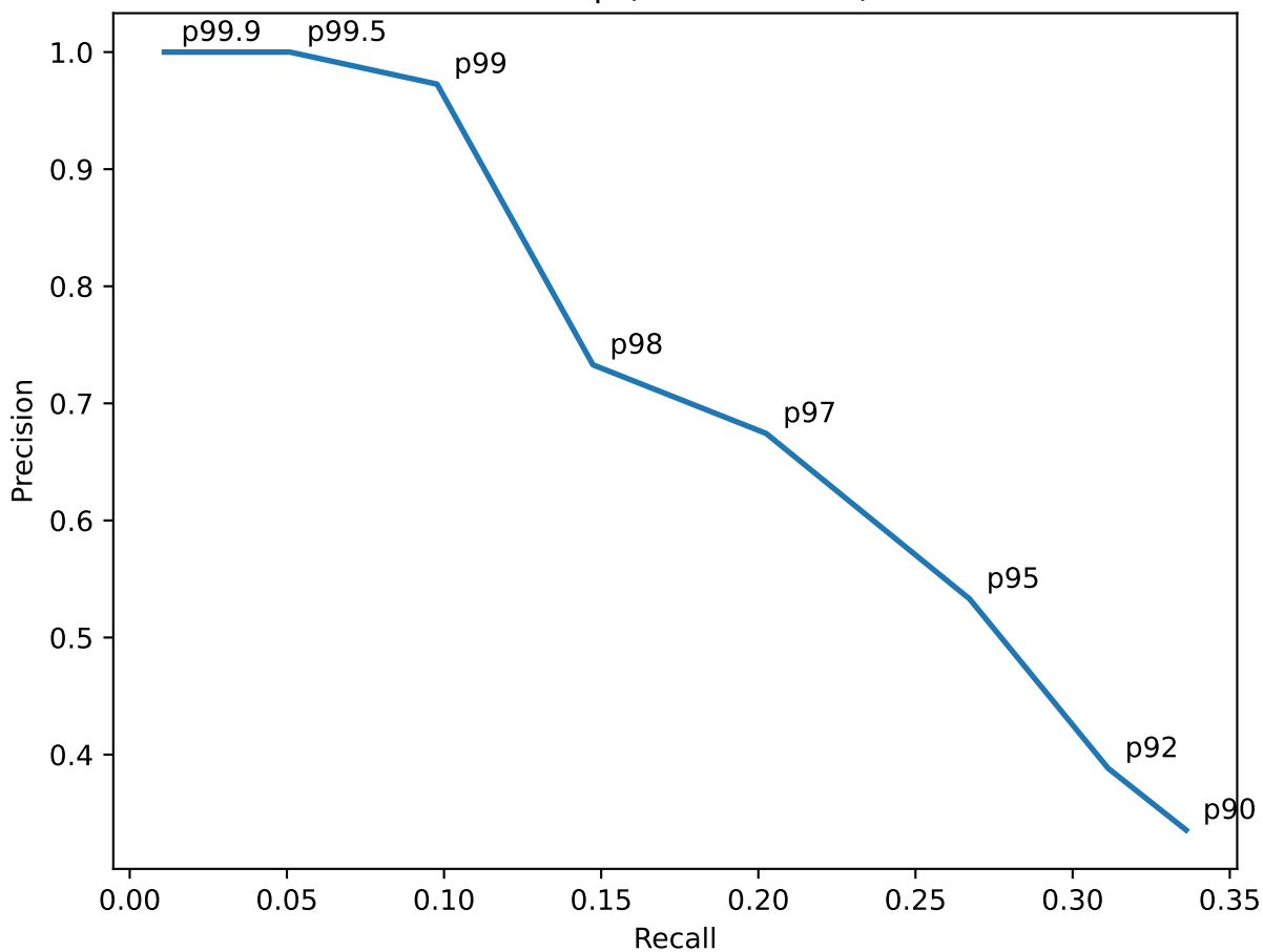
Isolation Forest - Percentile Sweep (window=48h): Precision-Recall trade-off
