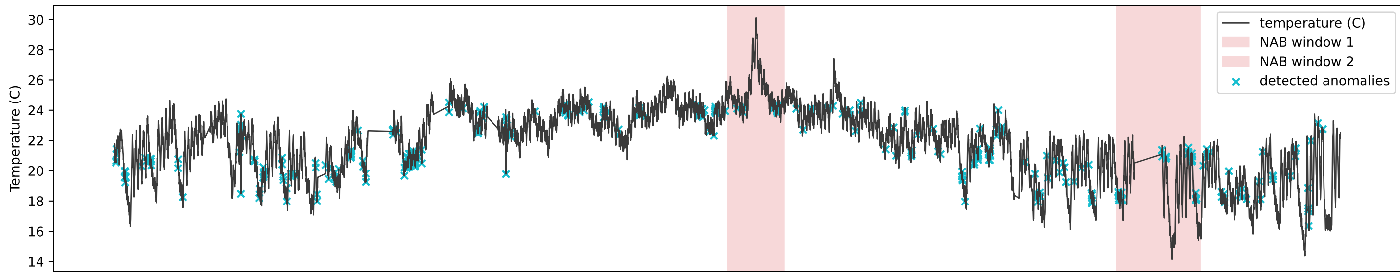
LOF - GT vs Detected (window=6h, k=20, p95) (A) NAB windows vs detector alarms
