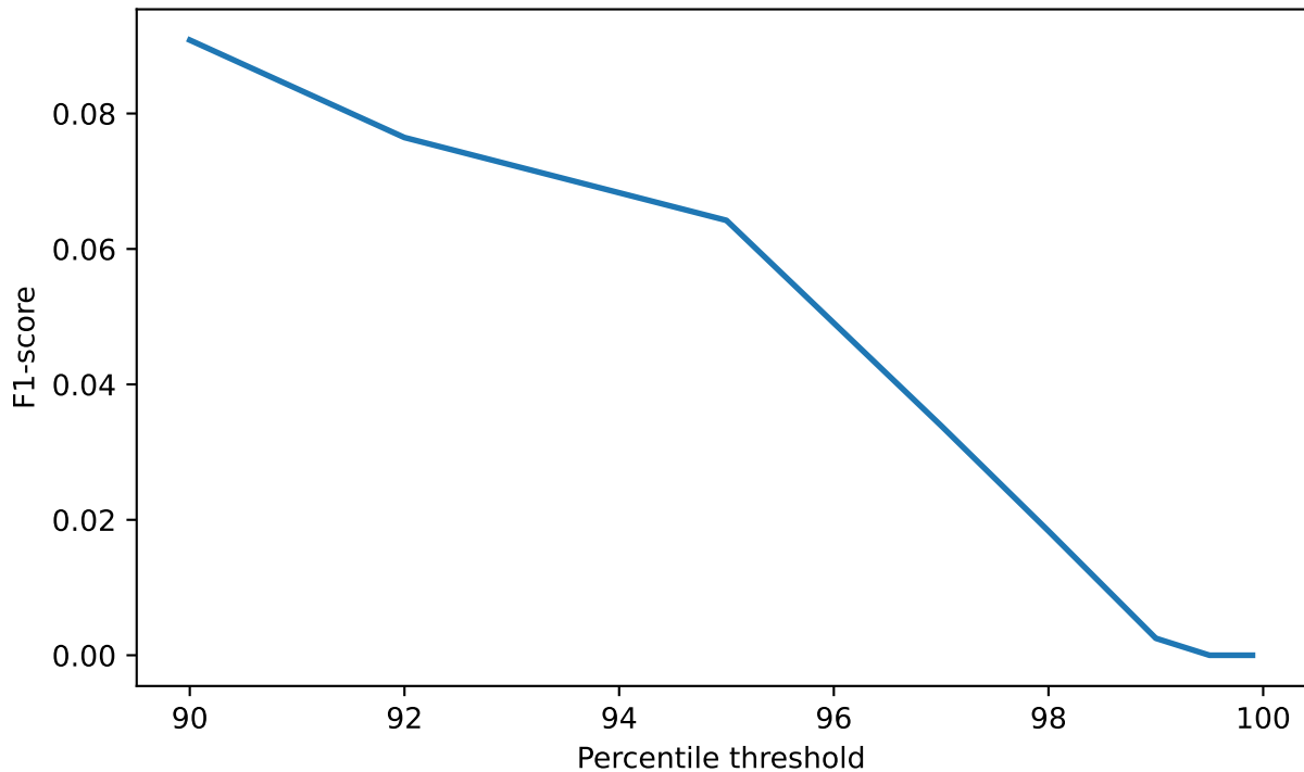
LOF - Percentile Sweep (window=6h, k=20): F1-score vs percentile threshold
