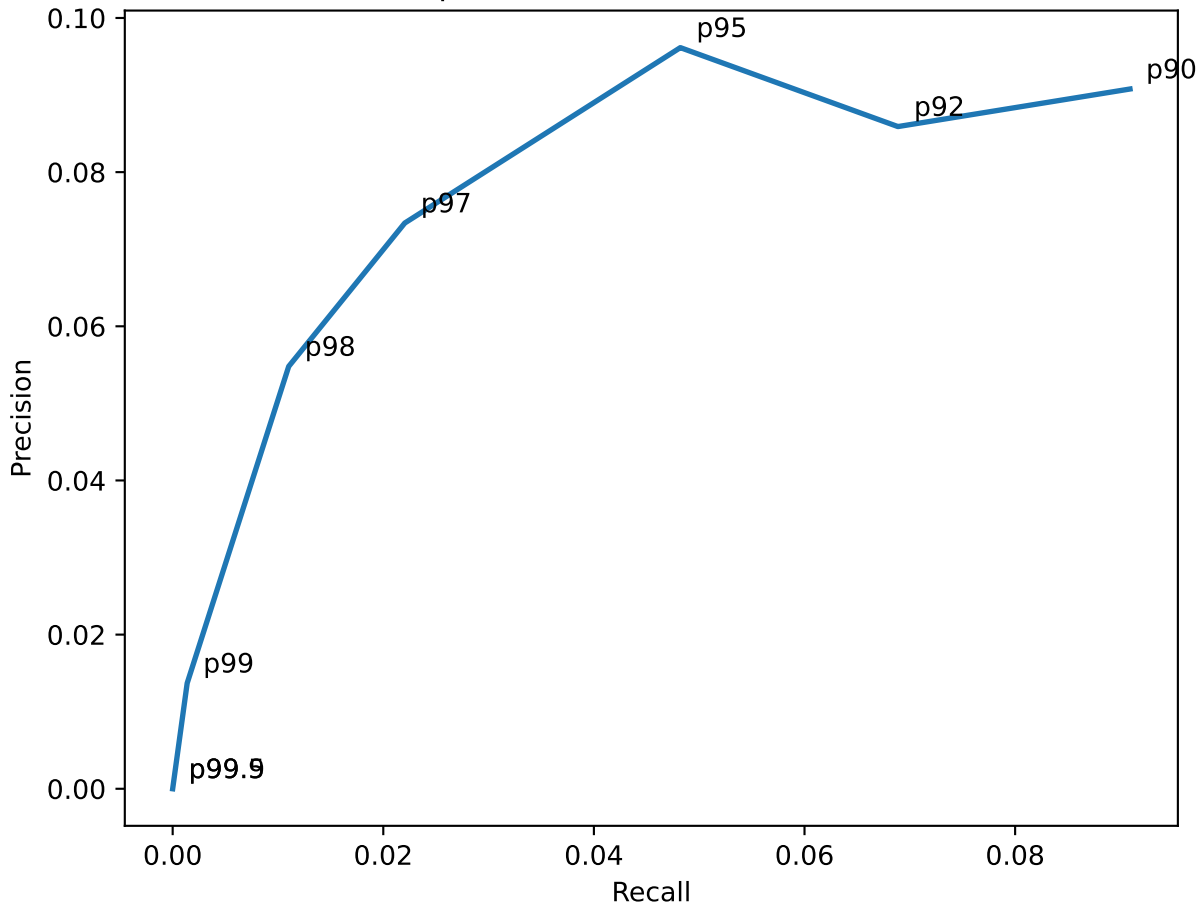
LOF - Percentile Sweep (window=6h, k=20): Precision-Recall trade-off
