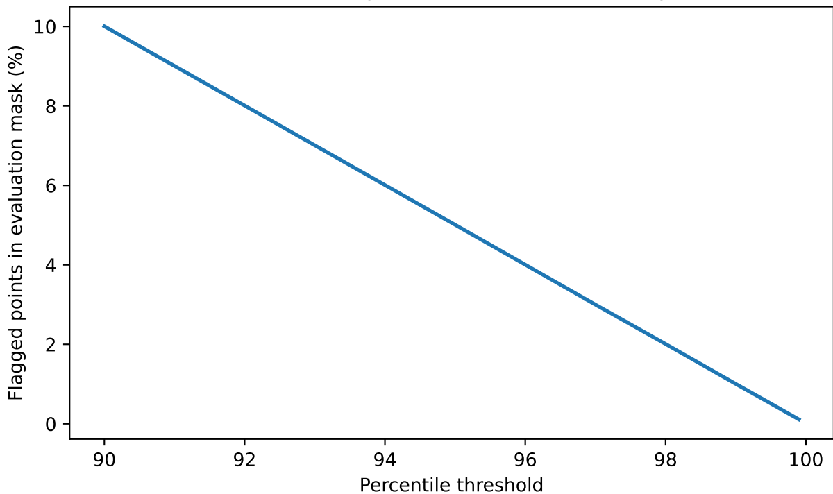
Matrix Profile - Percentile Sweep (m=12h): Alarm rate vs percentile threshold
