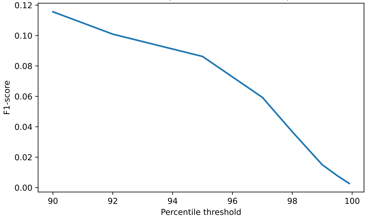
Matrix Profile - Percentile Sweep (m=12h): F1-score vs percentile threshold
