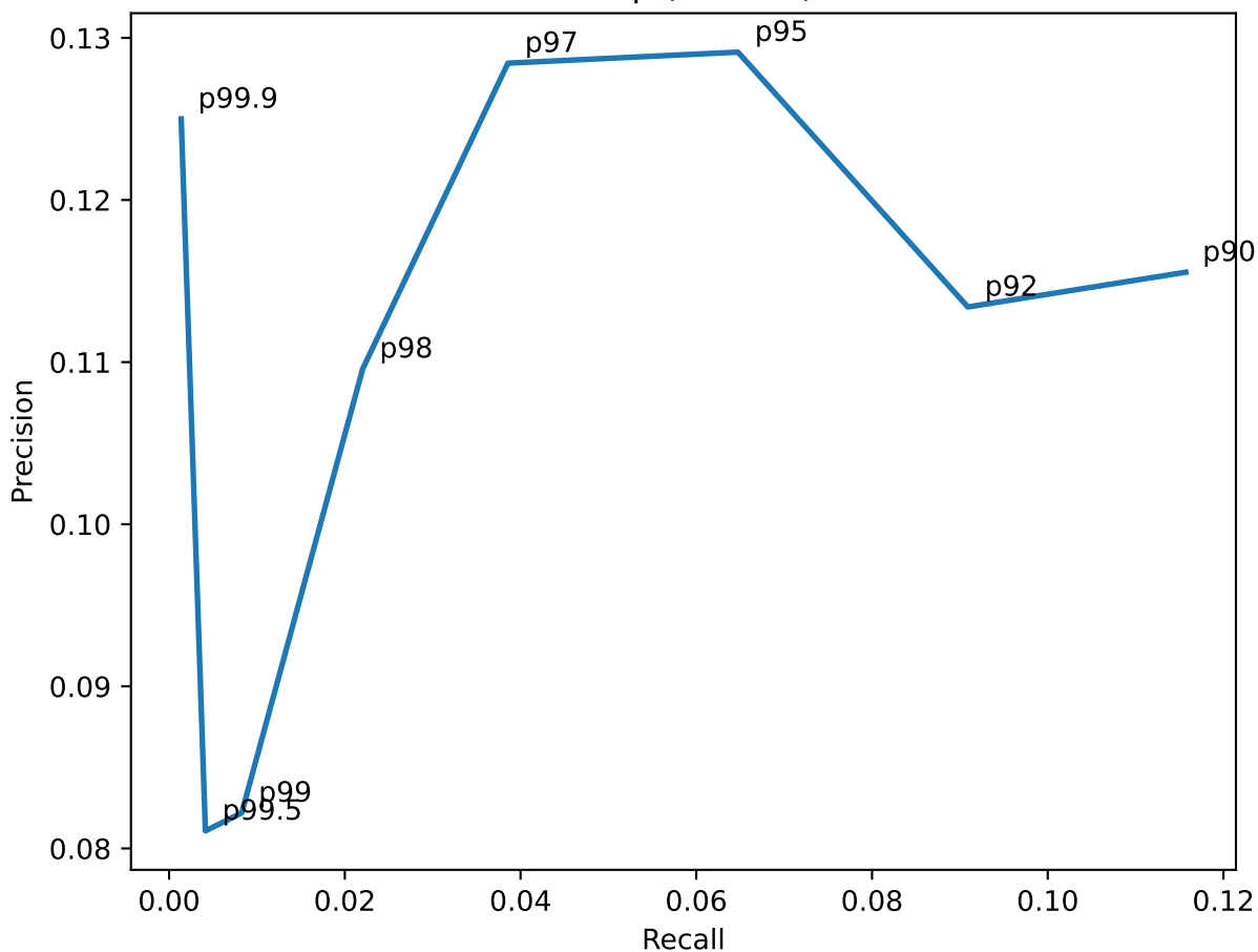
Matrix Profile - Percentile Sweep (m=12h): Precision-Recall trade-off
