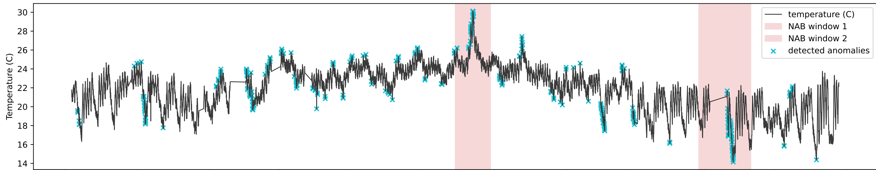
Rolling Z-score - GT vs Detected (window=168h, p95) (A) NAB windows vs detector alarms
