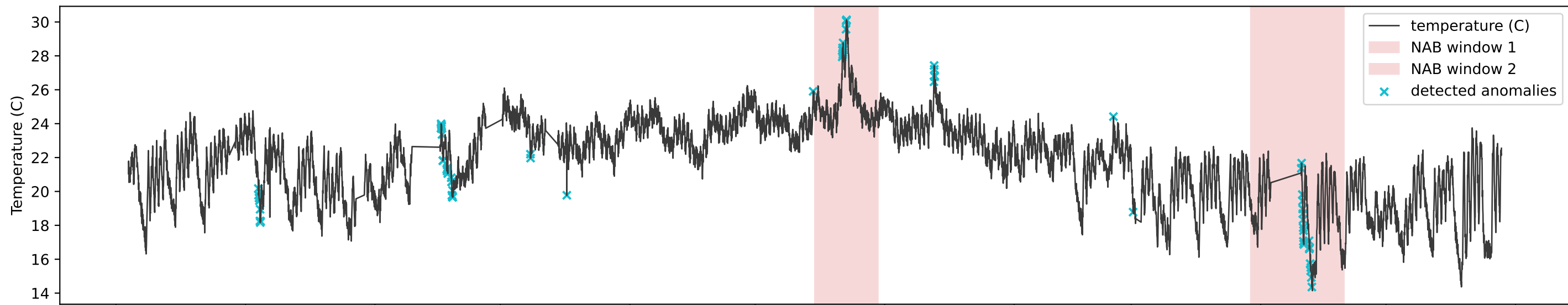
Rolling Z-score - GT vs Detected (window=168h, p99) (A) NAB windows vs detector alarms
