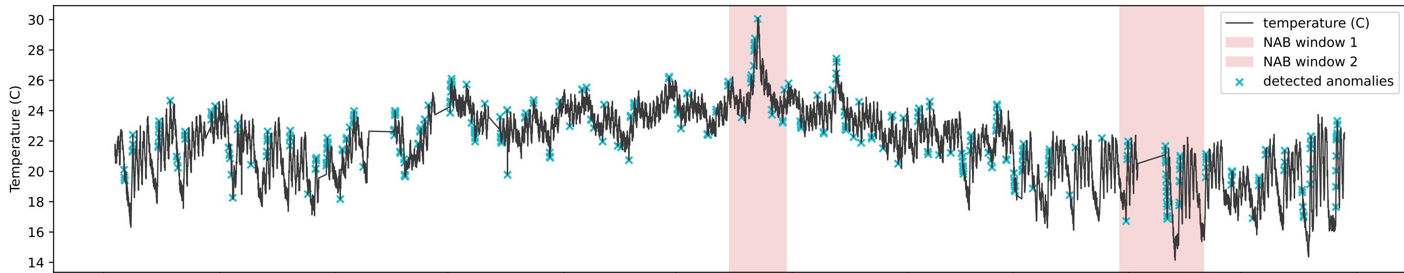
Rolling Z-score - GT vs Detected (window=48h, p95) (A) NAB windows vs detector alarms
