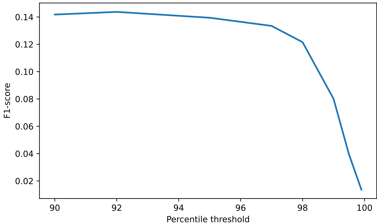
Rolling Z-score - Percentile Sweep (window=168h): F1-score vs percentile threshold
