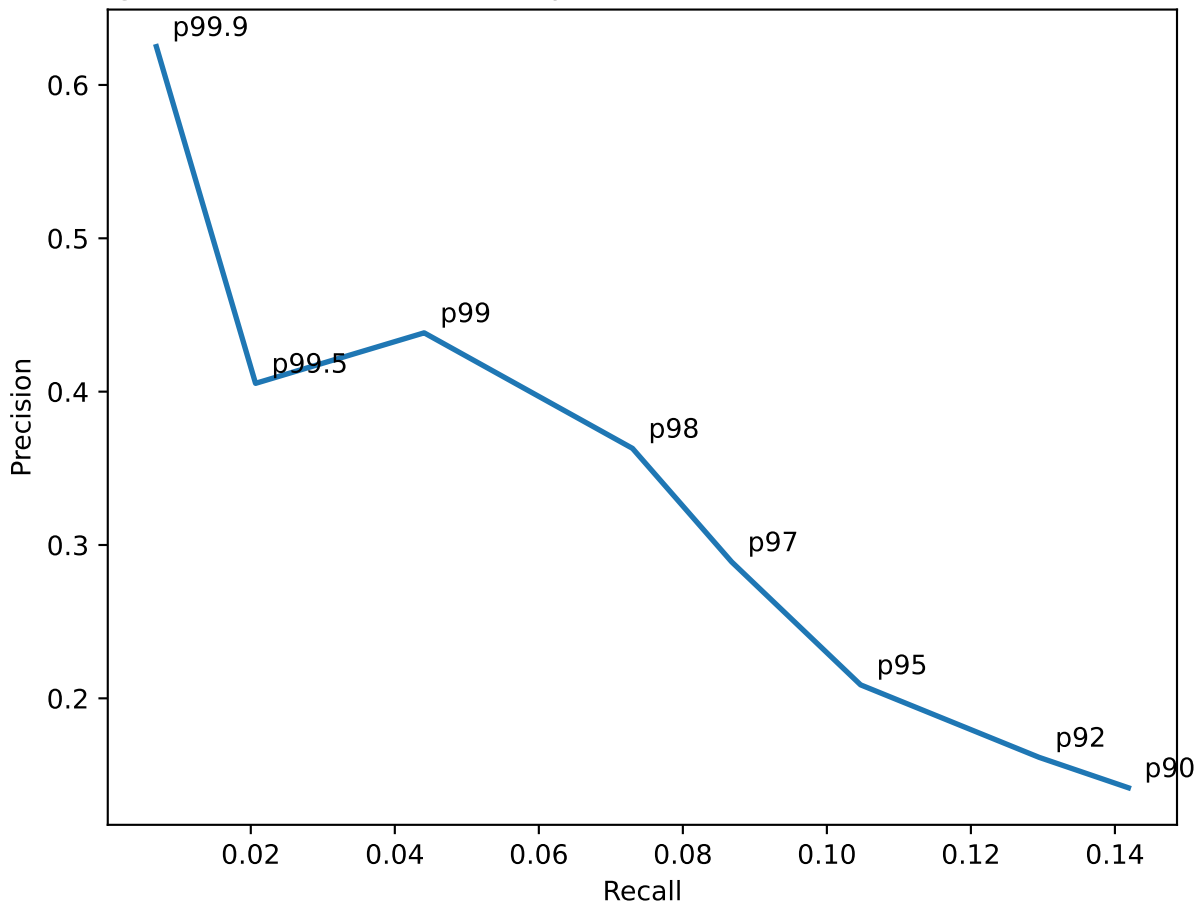
Rolling Z-score - Percentile Sweep (window=168h): Precision-Recall trade-off
