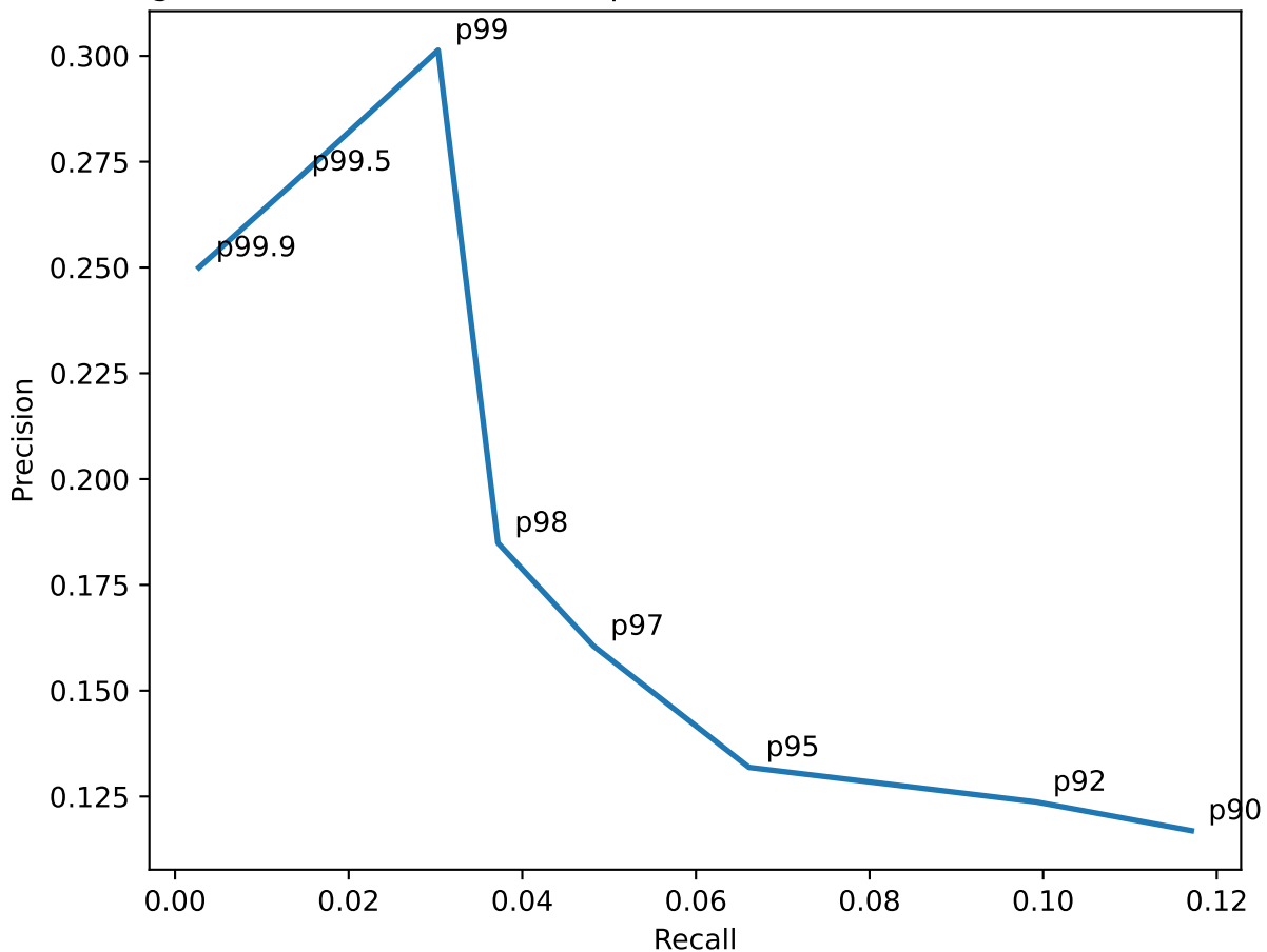
Rolling Z-score - Percentile Sweep (window=48h): Precision-Recall trade-off
