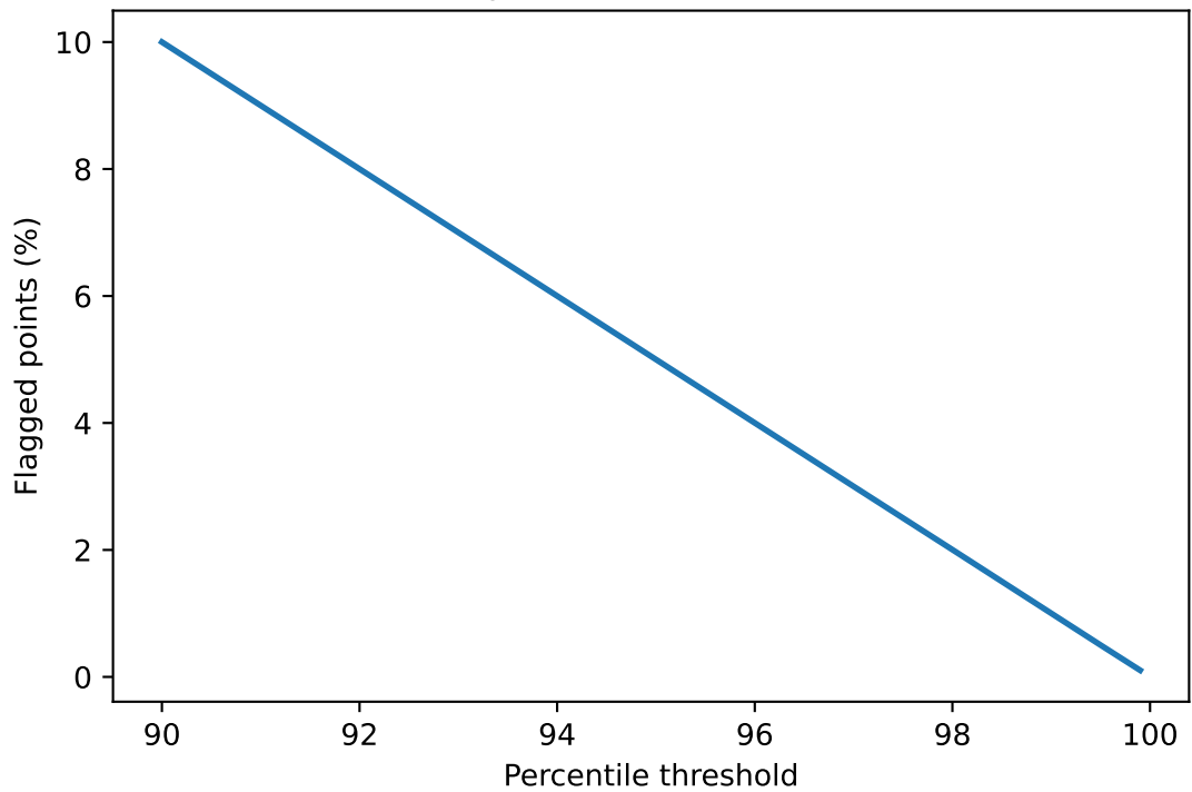
Isolation Forest: Alarm rate vs percentile threshold (window=360, scaled=True)
