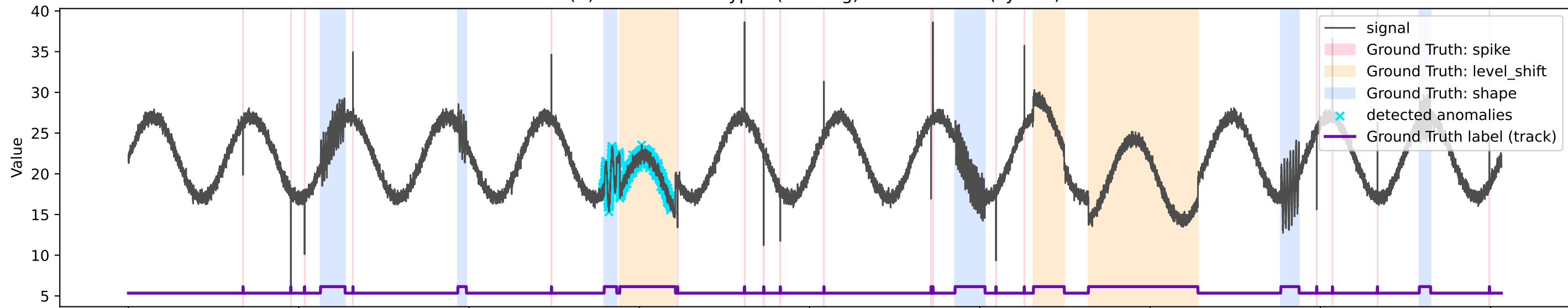
Matrix Profile — GT vs Detected + TP/FP/FN (m=1440, p95.0)
