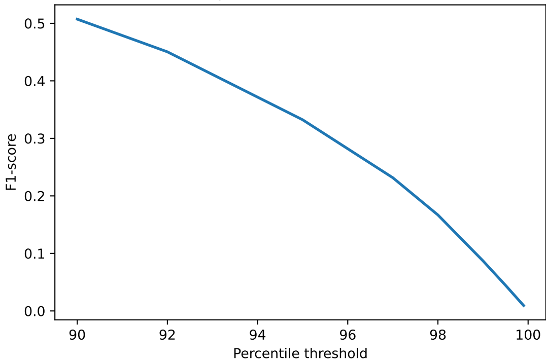
Isolation Forest: F1-score vs percentile threshold (window=360, scaled=True)
