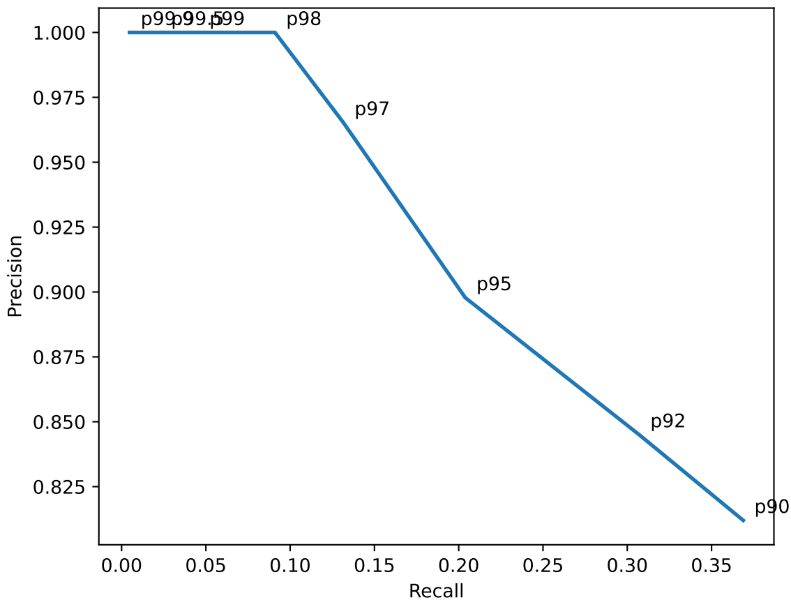
Isolation Forest: Precision-Recall trade-off (window=360, scaled=True)
